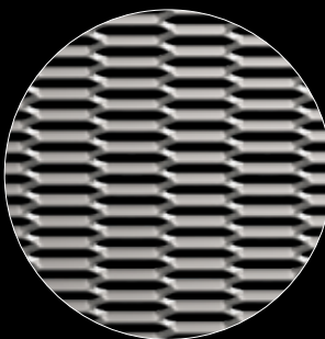
XP303 STRAND WIDTH: 6 mm OVERALL THICKNESS: 9.5 mm OPEN AREA: 42.6% DIMENSIONS (W x H): 1000 x No limit / 1500 x No limit
