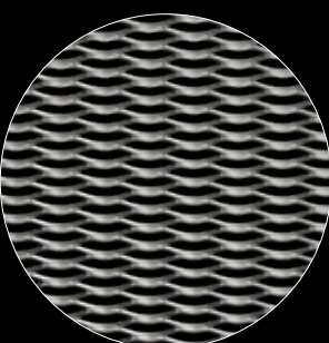
XP109 STRAND WIDTH: 4 mm OVERALL THICKNESS: 7.5 mm OPEN AREA: 59.4% DIMENSIONS (W x H): 1000 x No limit / 1500 x No limit
