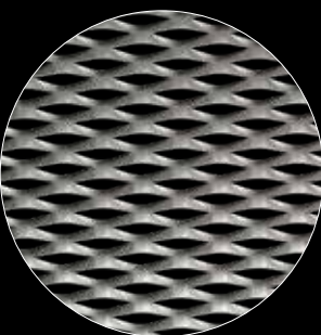
XP105 STRAND WIDTH: 8 mm OVERALL THICKNESS: 11 mm OPEN AREA: 49.3% DIMENSIONS (W x H): 1000 x No limit / 1500 x No limit
