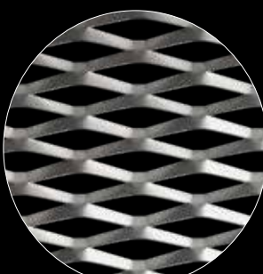
XP201 STRAND WIDTH: 14 mm OVERALL THICKNESS: 18 mm OPEN AREA: 50.1% DIMENSIONS (W x H): 1000 x No limit / 1500 x No limit
