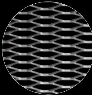
XP206 STRAND WIDTH: 6 mm OVERALL THICKNESS: 11 mm OPEN AREA: 67.5% DIMENSIONS (W x H): 1000 x No limit / 1500 x No limit
