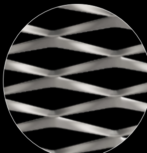
XP401 STRAND WIDTH: 20 mm OVERALL THICKNESS: 28 mm OPEN AREA: 62.7% DIMENSIONS (W x H): 1000 x No limit / 1500 x No limit
