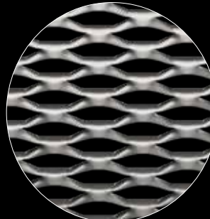
XP333 STRAND WIDTH: 11.5 mm OVERALL THICKNESS: 15.5 mm OPEN AREA: 58.6 % DIMENSIONS (W x H): 1000 x No limit / 1500 x No limit
