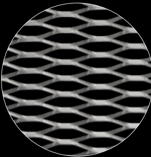
XP204 STRAND WIDTH: 8 mm OVERALL THICKNESS: 14 mm OPEN AREA: 64.3% DIMENSIONS (W x H): 1000 x No limit / 1500 x No limit
