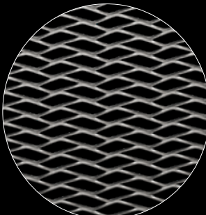
XP106 STRAND WIDTH: 4 mm OVERALL THICKNESS: 7.8 mm OPEN AREA: 62.4% DIMENSIONS (W x H): 1000 x No limit / 1500 x No limit
