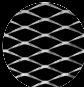
XP503 STRAND WIDTH: 9 mm OVERALL THICKNESS: 14 mm OPEN AREA: 55% DIMENSIONS (W x H): 1000 x No limit / 1500 x No limit
