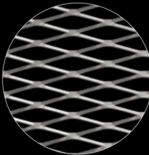
XP203 STRAND WIDTH: 8 mm OVERALL THICKNESS: 13.5 mm OPEN AREA: 65.8% DIMENSIONS (W x H): 1000 x No limit / 1500 x No limit
