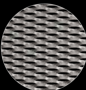
XP110 STRAND WIDTH: 8 mm OVERALL THICKNESS: 10.5 mm OPEN AREA: 37% DIMENSIONS (W x H): 1000 x No limit / 1500 x No limit
