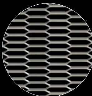
XP304 STRAND WIDTH: 6 mm OVERALL THICKNESS: 10.5 mm OPEN AREA: 45.5% DIMENSIONS (W x H): 1000 x No limit / 1500 x No limit
