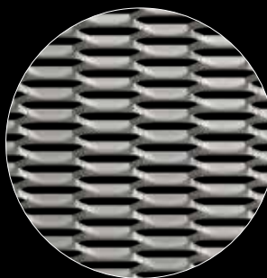
XP302 STRAND WIDTH: 8 mm OVERALL THICKNESS: 11.5 mm OPEN AREA: 56.6% DIMENSIONS (W x H): 1000 x No limit / 1500 x No limit
