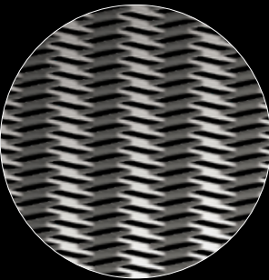
XP101 STRAND WIDTH: 4 mm OVERALL THICKNESS: 7.5 mm OPEN AREA: 49.3% DIMENSIONS (W x H): 1000 x No limit / 1500 x No limit
