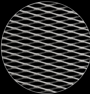
XP104 STRAND WIDTH: 4.5 mm OVERALL THICKNESS: 8 mm OPEN AREA: 67.7% DIMENSIONS (W x H): 1000 x No limit / 1500 x No limit
