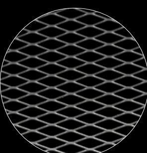
XP113 STRAND WIDTH: 4 mm OVERALL THICKNESS: 8 mm OPEN AREA: 68.7% DIMENSIONS (W x H): 1000 x No limit / 1500 x No limit
