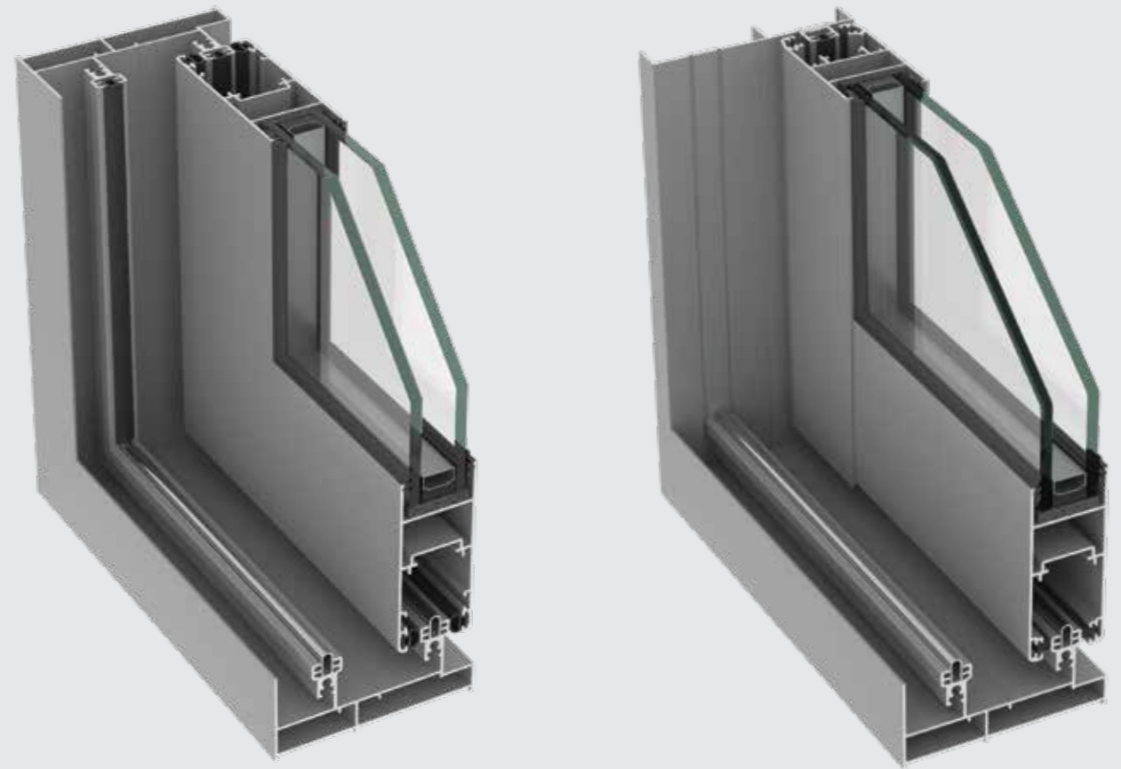
Sash profiles for 45° and 90° assembling.
