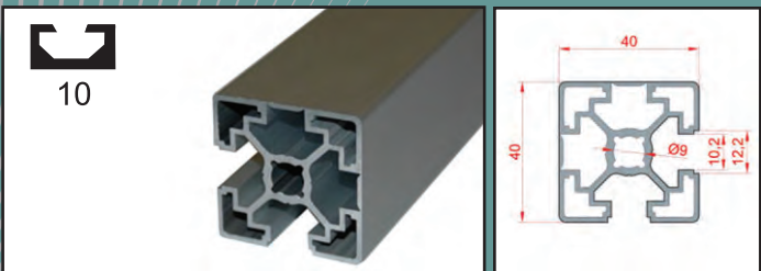
40X40 Closed profile
