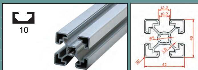
40X40 profile
