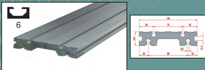
22X140 surface coating profile
