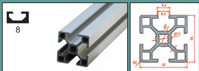
35X35 profile
