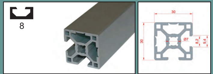
30X30 Closed profile
