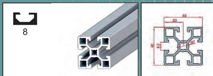
40X40 Heavy profile
