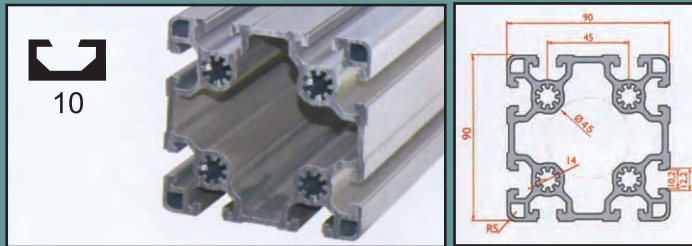
90X90 profile
