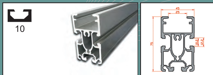
45X75 Conveyor profile
