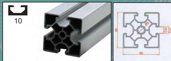
60X60 profile
