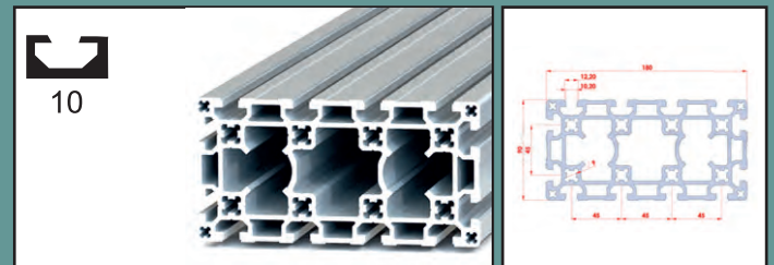
90X180 Heavy profile
