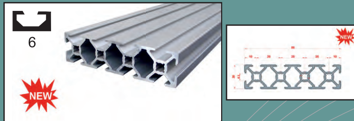
20X80 profile
