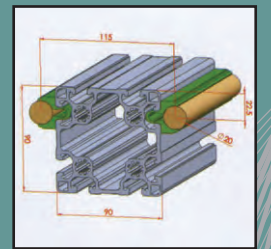
Rod shaft support profile Ø 12-16-20-25-30-40 (without hole)
