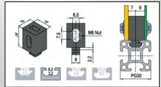
Panel Mounting Block 8
