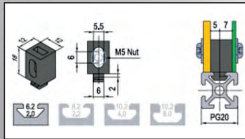
Panel Mounting Block 6
