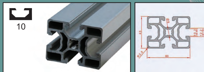
45X60 profile
