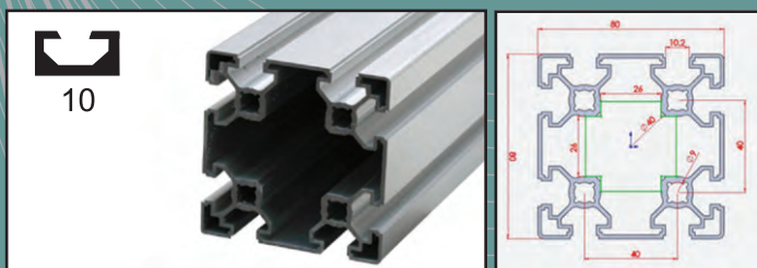
80X80 profile
