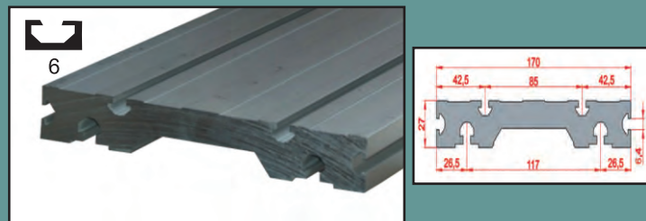
27X170 surface coating profile
