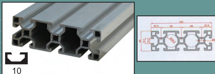
45X135 profile
