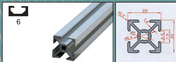
20X20 profile
