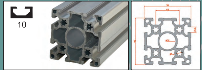
90X90 Heavy profile
