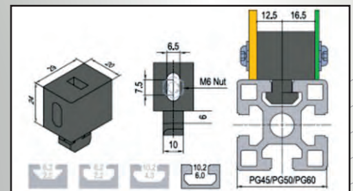
Panel Mounting Block 10-6
