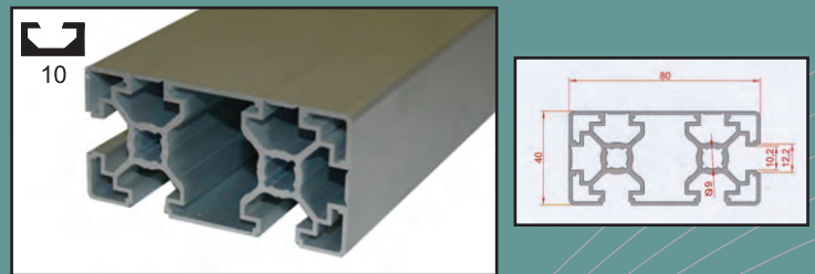
40X80 Closed profile
