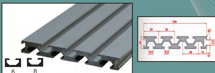
15X120 surface coating profile
