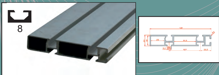
23X127 Conveyor profile
