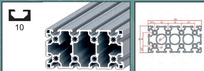
90X180 profile
