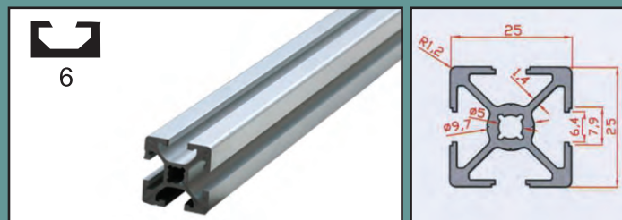
25X25 profile
