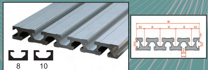
22,5X180 surface coating profile
