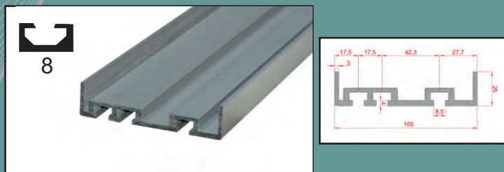
25X105 & 25X150 Conveyor profile
