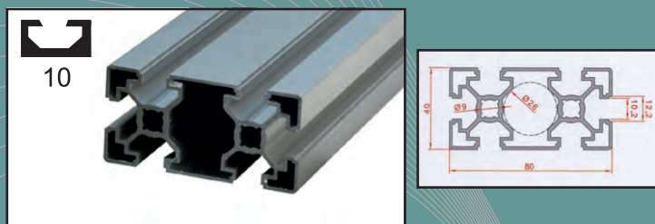
40X80 profile
