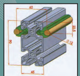
Rod shaft support profile Ø 12-16-20-25-30-40 (without hole)
